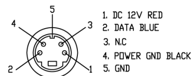
4PIN JDAB FEMALE
