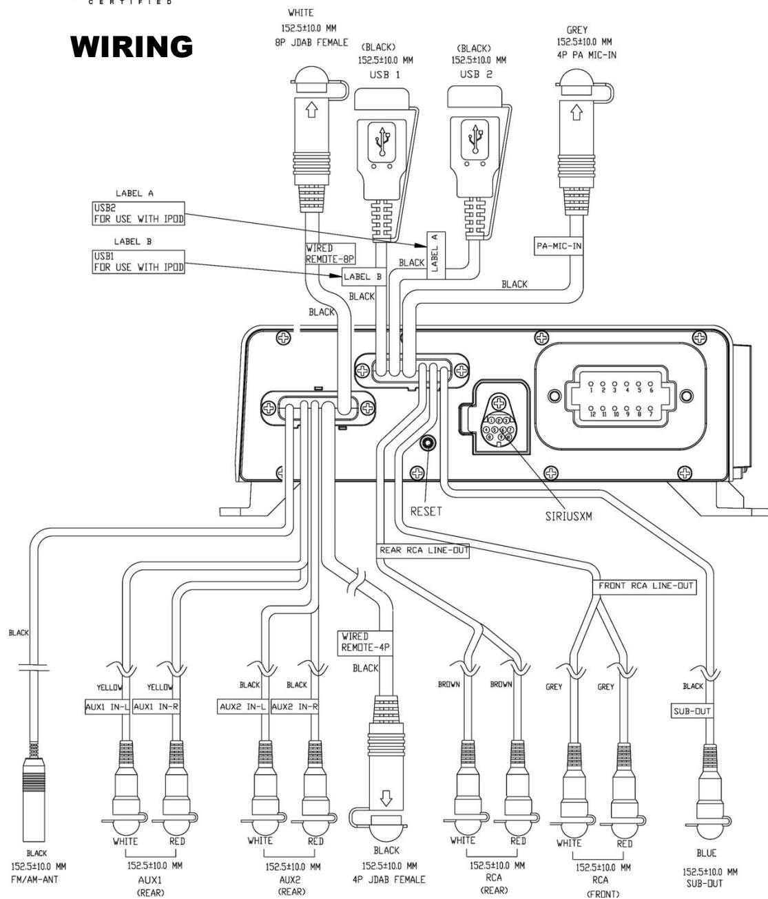
(8 PIN JDAB FEMALE)
