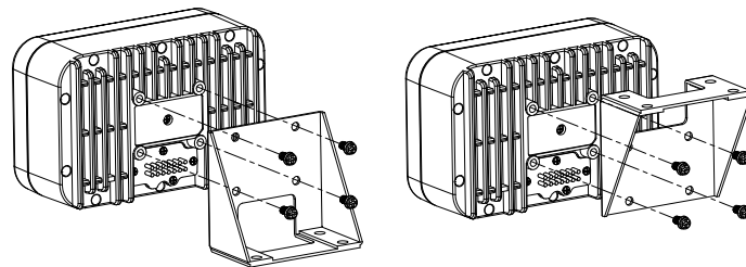
Regular Mounting
