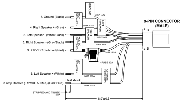
VIEW B-B WIRE INSERTION VIEW
