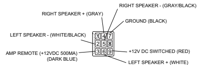
VIEW A-A WIRE INSERTION VIEW
