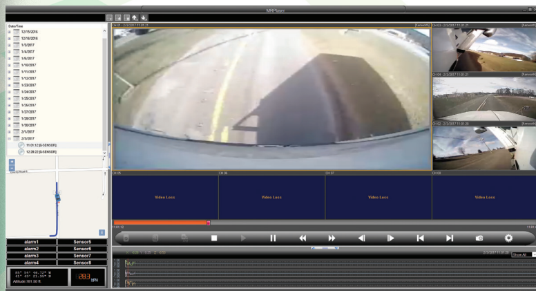
Software Interface
